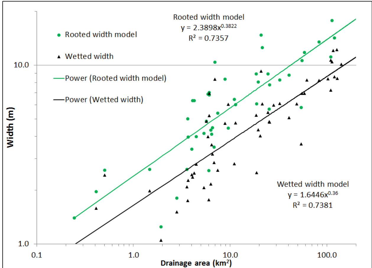
Figure 18. Rooted width and wetted width models using FWMIS data from Racehorse and Dutch Creeks. Note: only wetted widths measured during the August and September baseflow season were used.
